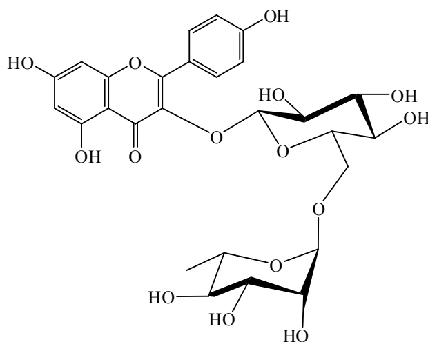
Kaempférol-3-O-[\alpha-L-rhamnopyranosyl-(1→6)-\beta-D-glucopyranoside]
