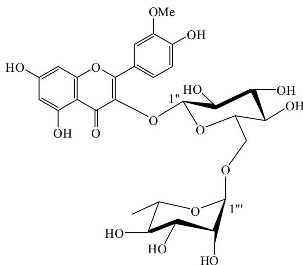
isorhamnetin-3-O-[\alpha-L-rhamnopyranosyl-(1→6)-\beta-D-glucopyranoside]
