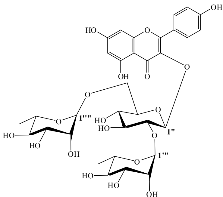
Kaempférol-3-O-[2,6-di-O-α-L-rhamnopyranosyl-β-D-glucopyranoside]
