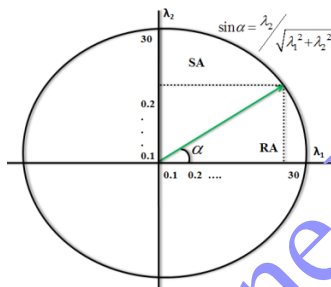
Figure 5. Allocation strategy.
