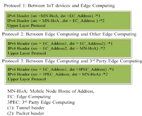
Figure 11. Communication protocols
